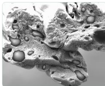
Figure 3: Capsules in viscose fibre [6]
