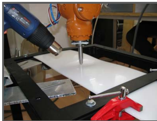
Figure 7. Polyethilen sheet forming by KUKA KR6 robot
