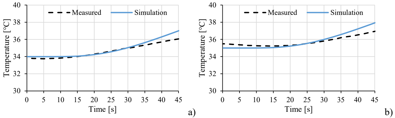
Fig. 8. Comparison of the measured and the simulated mould insert volumetric temperature a) 200 bar holding pressure, b) 300 bar holding pressure.
