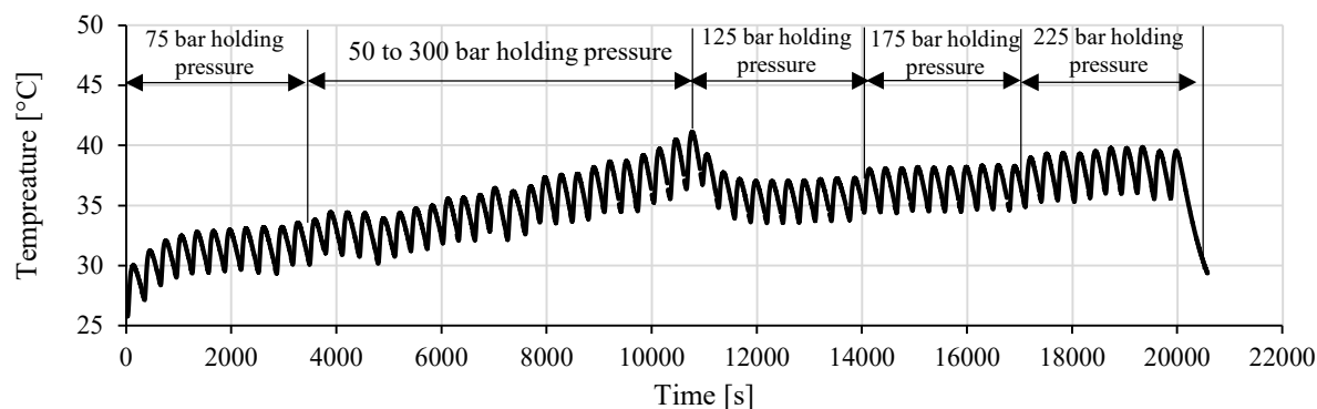
Fig. 5. The volumetric temperature of the mould insert measured by the thermocouple.
