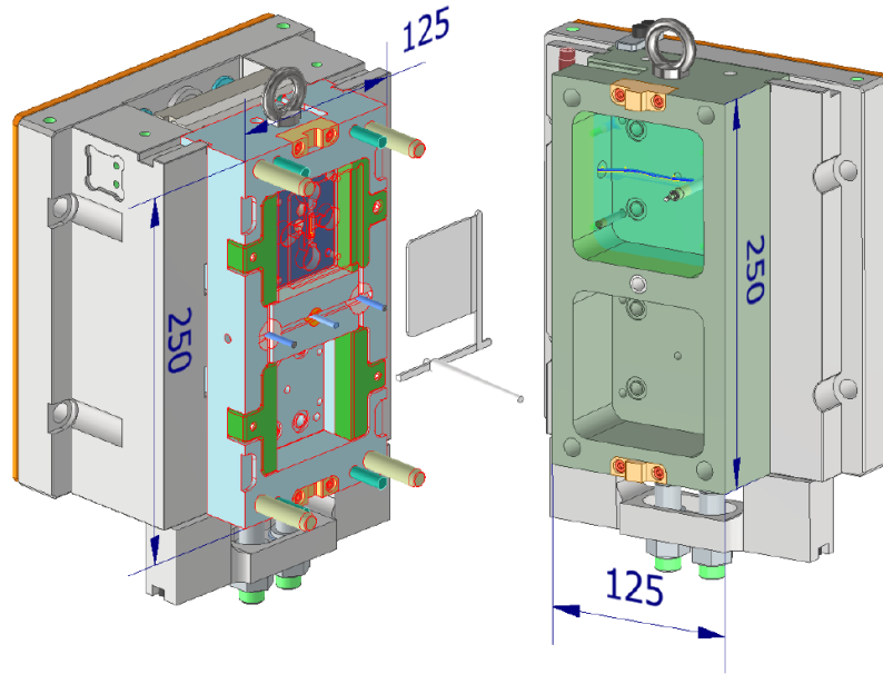
Fig.1. The test mould.
