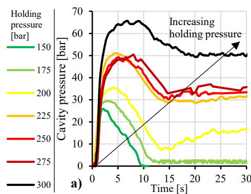
Fig. 4. The cavity pressure results at increasing holding pressure.
