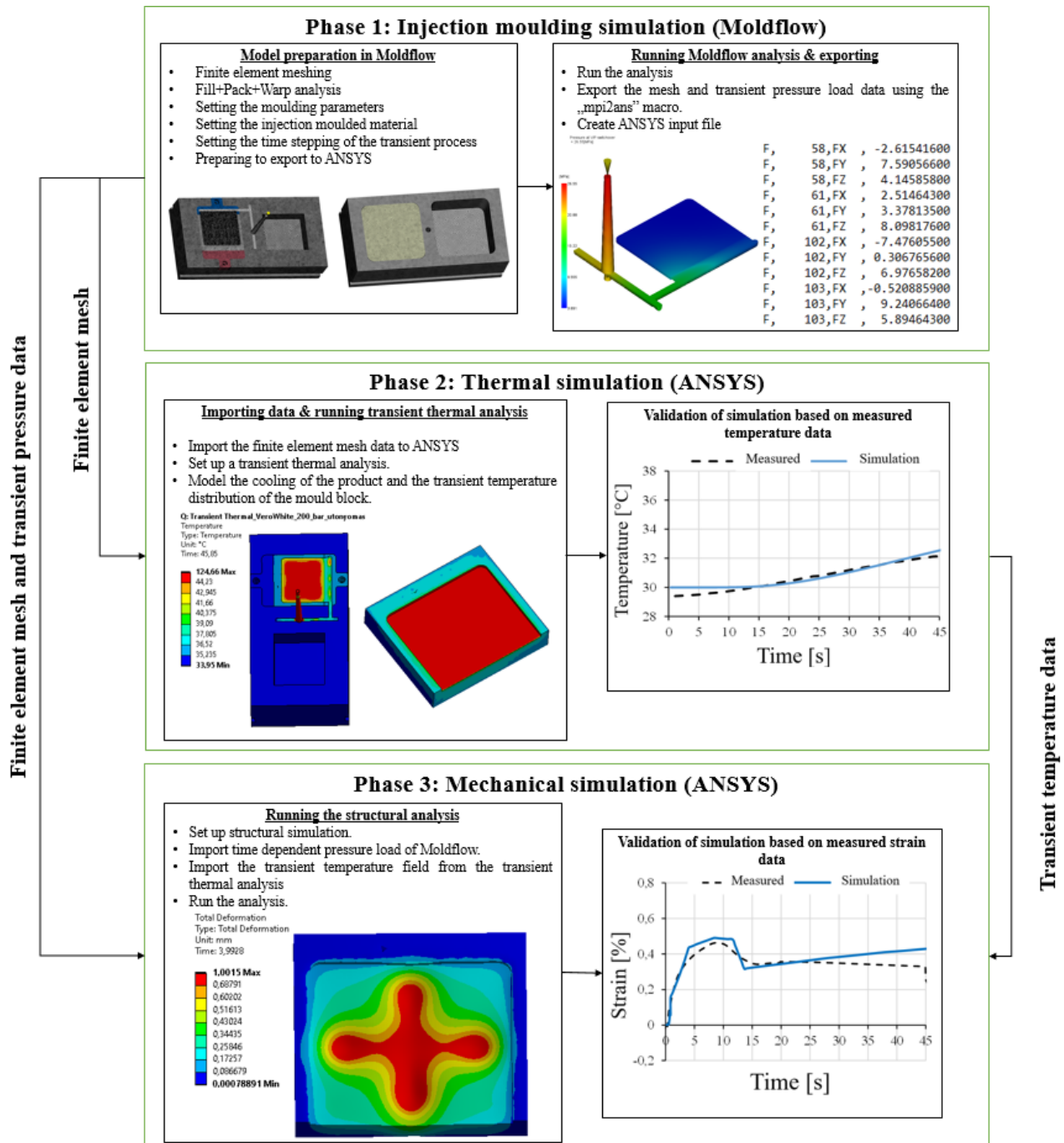
Fig. 7. Workflow of the coupled simulation method.
