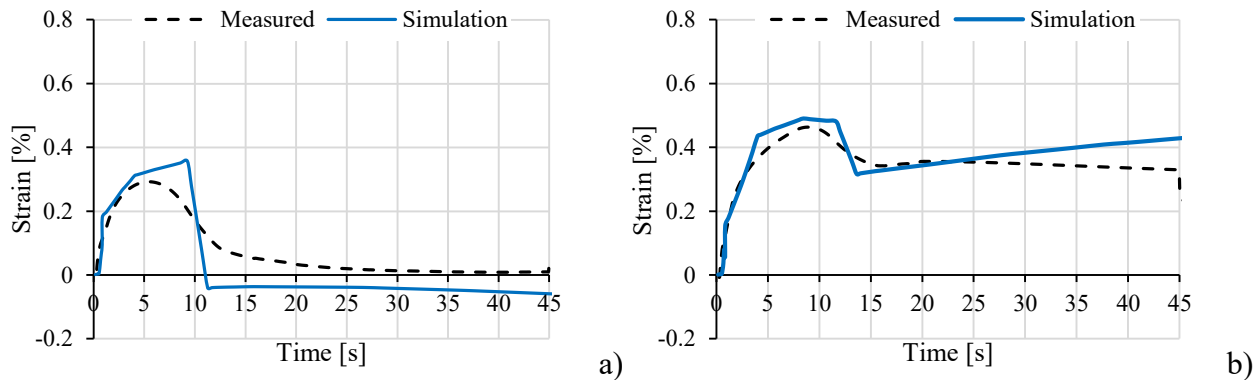
Fig. 9. Comparison of the measured and the simulated mould insert strain a) 200 bar holding pressure, b) 300 bar holding pressure.
