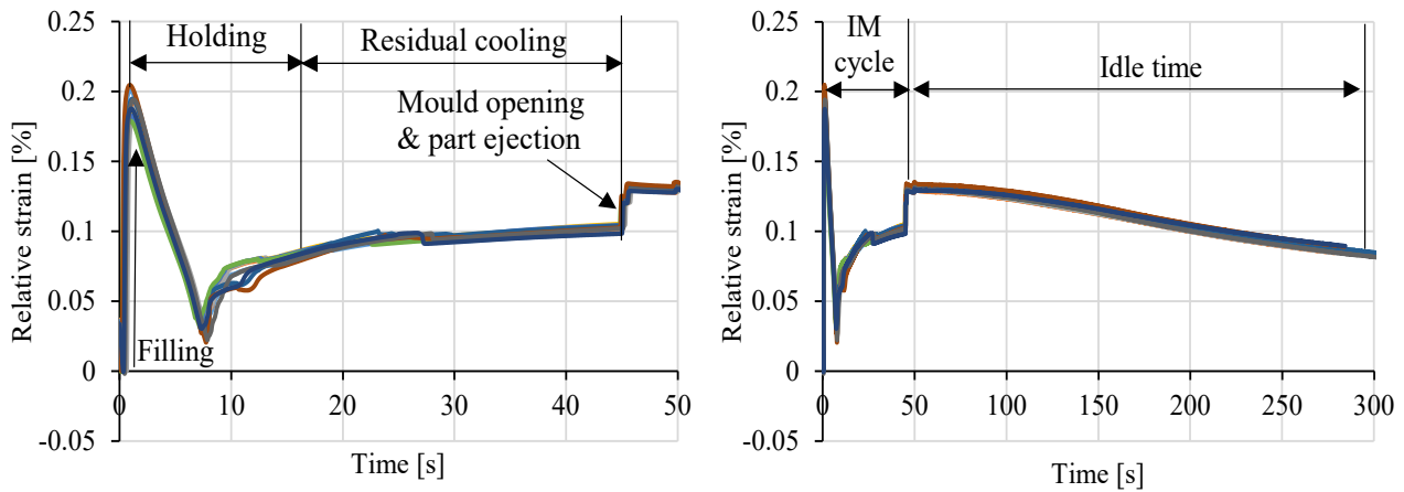
Fig. 2. The relative strain results at 75 bar holding pressure.
