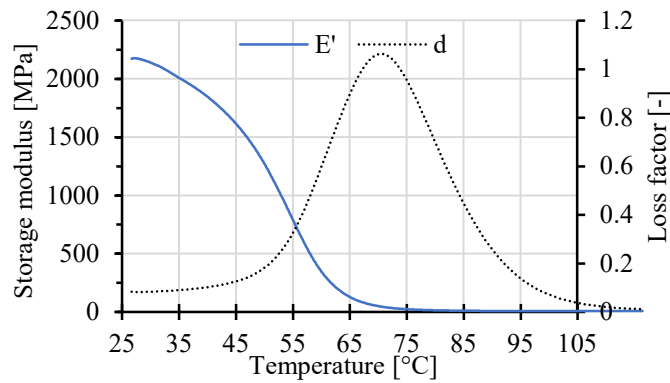
Fig. 6. The storage modulus and loss factor of the VeroWhite material.
