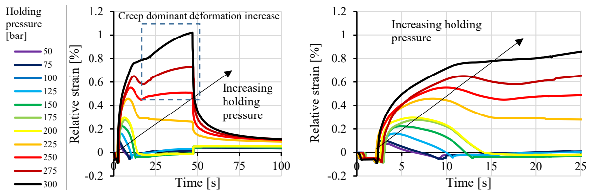
Fig. 3. The relative strain results at increasing holding pressure.
