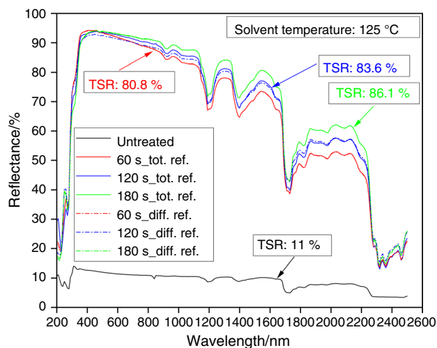
Fig. 4 Total and diffuse reflectance of solvent-treated PP sheets after different immersion times (60, 120, 180 s) compared to the untreated sample
