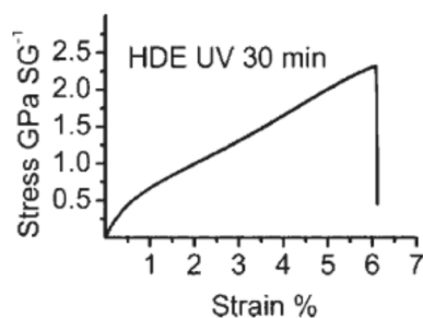
Fig. 2.12. Non-linear response of carbon nanotube fibre. The unit \text{GPa SG}^{-1} ( \text{SG} = \text{specific gravity} ) is equal to \text{GPa cm}^3/\text{g} [41].
