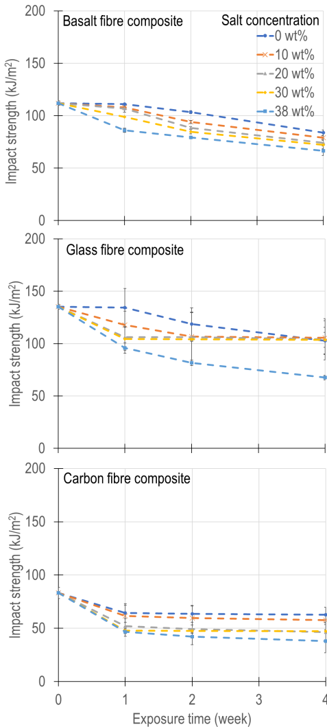
Figure 9. Impact strength values of composites determined by the Charpy impact test
