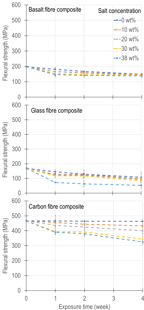
Figure 7 Flexural strength values of composites determined during bending tests
