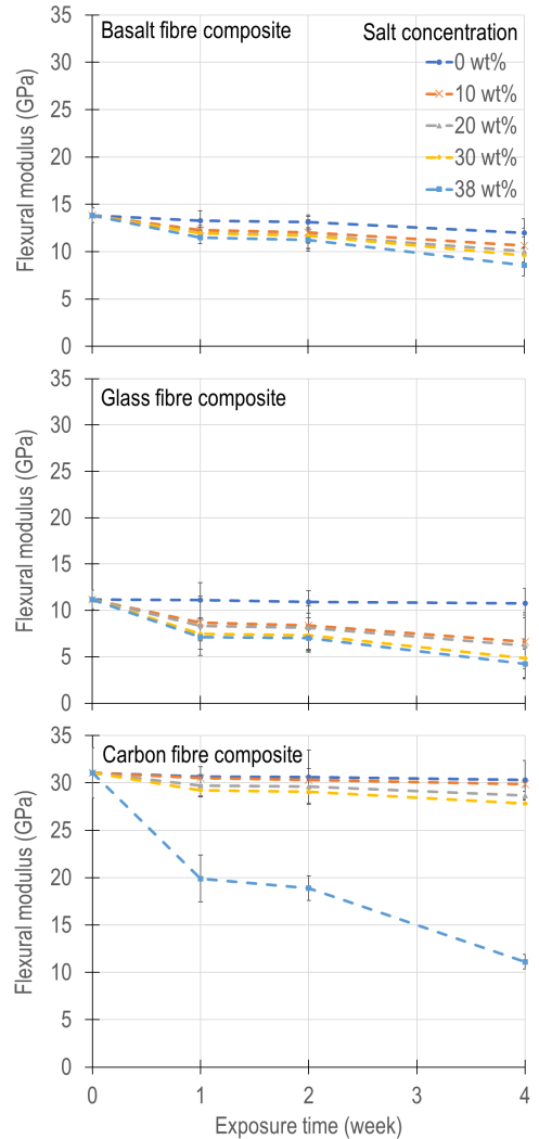
Figure 8 Flexural elastic modulus values of composites determined by bending tests
