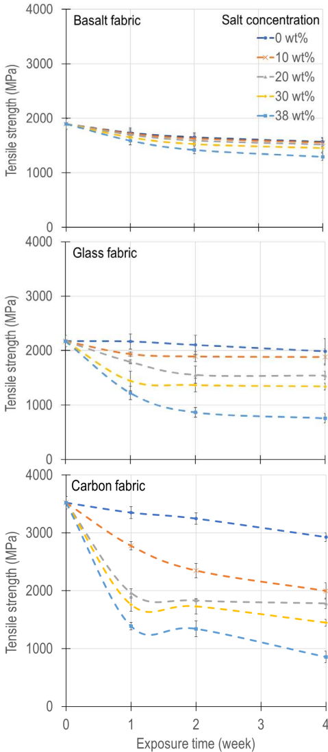
Figure 1 The effect of salt-water on the tensile strength of reinforcements
