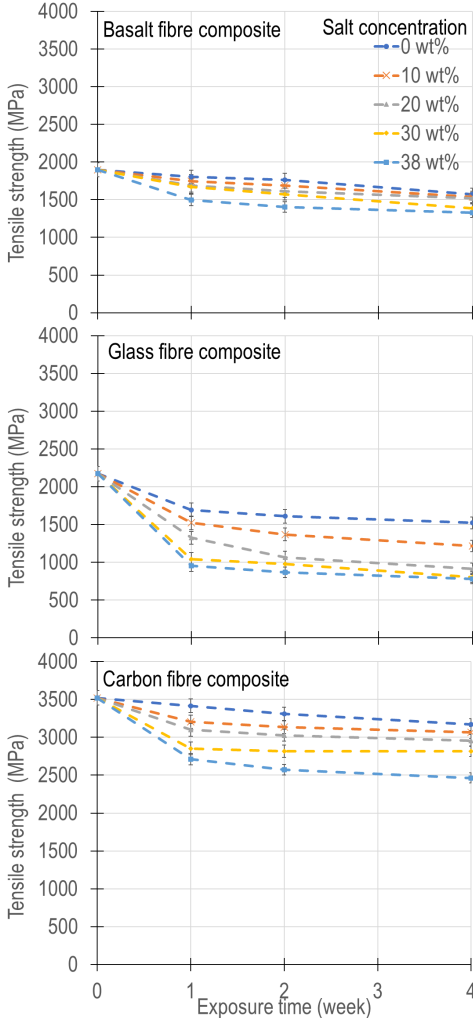
Figure 5 Tensile strength values of composites determined during the tensile test
