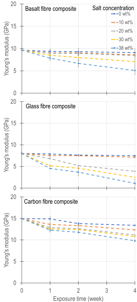
Figure 6 Tensile modulus of elasticity values of composites determined during tensile tests
