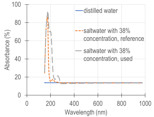
Figure 4 Results of ultraviolet spectroscopic studies
