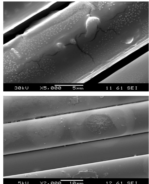
Figure 2 Damage of elemental basalt fibres by salt water treatment; 38% concentration 4 weeks (upper), 30% concentration 4 weeks (lower)
