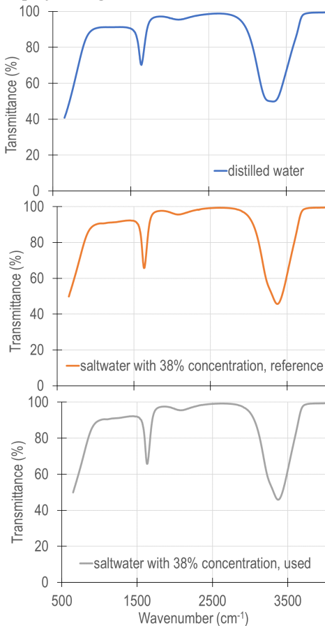
Figure 3 Results of Fourier transform infrared spectroscopic measurements
