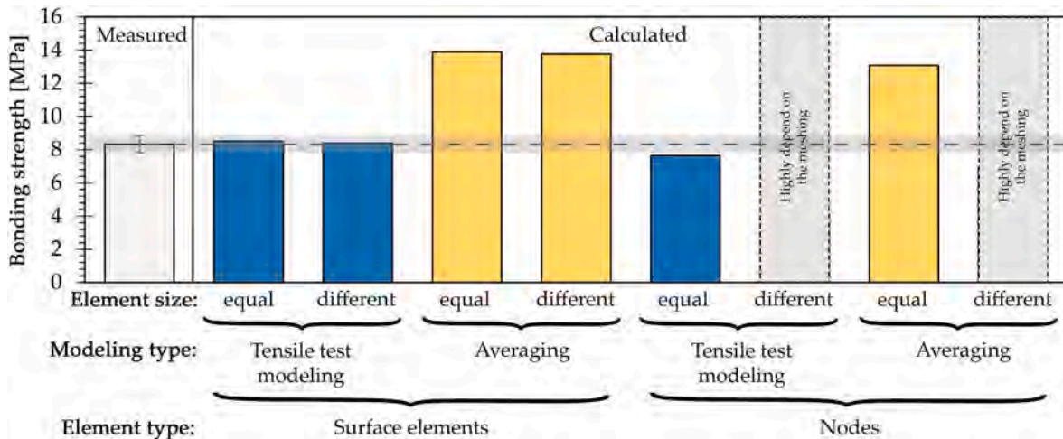
Fig. 26. Calculation method results for bonding strength with the measurement results (blue bar - results obtained by tensile test modeling, yellow bar - results obtained by averaging). (For interpretation of the references to colour in this figure legend, the reader is referred to the Web version of this article.)
