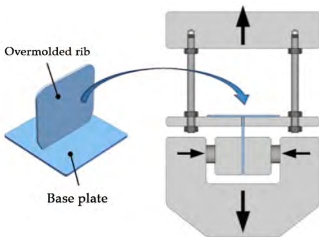
Fig. 4. Special grip for tensile tests.
