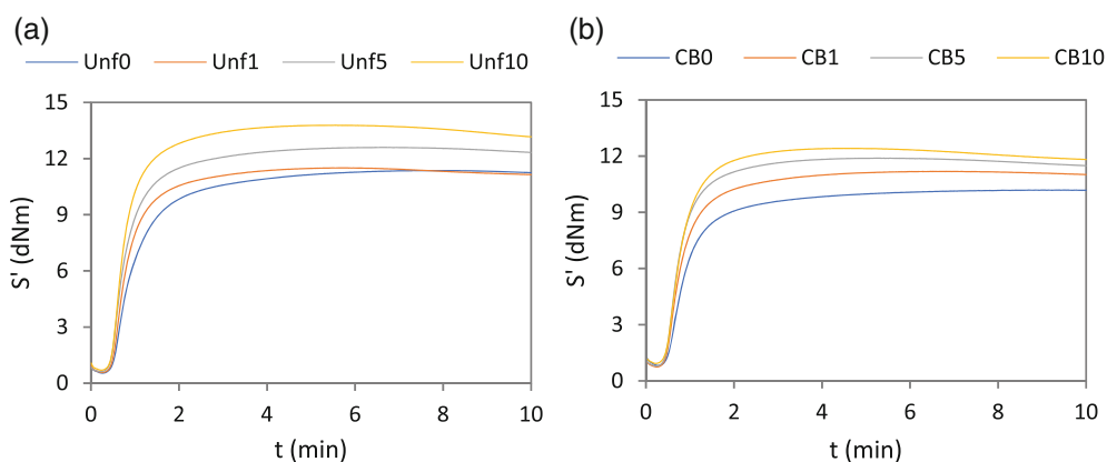
FIGURE 2 Curing curves for the unfilled (a) and carbon black filled (b) experimental sets. [Color figure can be viewed at wileyonlinelibrary.com ]
