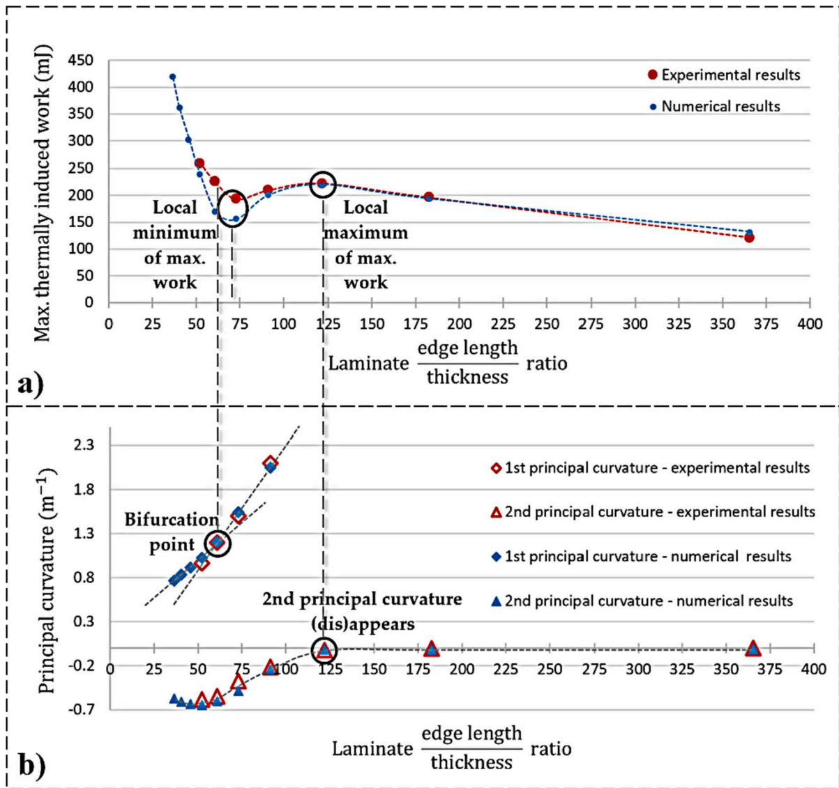
Fig. 7. Numerical and experimental results of the a) maximum thermally induced work and b) principal curvatures of the 190 mm × 190 mm [45 n /90 n /-75 n /-45 n ] laminates as a function of their dimensional ratio (constant 190 mm × 190 mm laminate).
