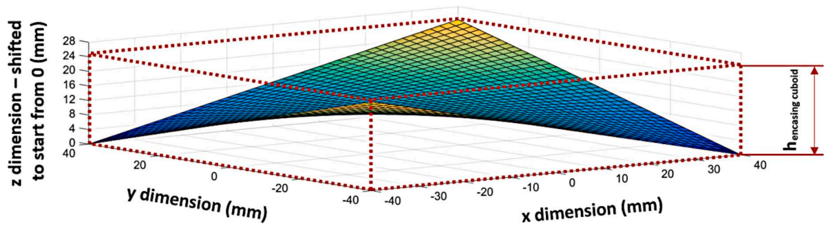
Fig. 1. Height of the enclosing cuboid ( h_{\text{encasing cuboid}} ) of a warped laminate.
