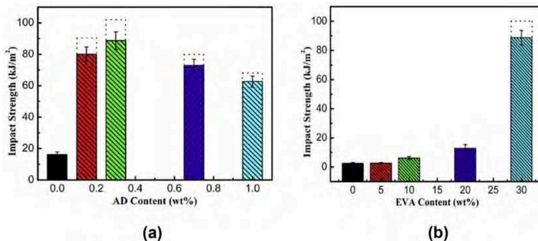
Fig. 20. The impact strength of PLA/EVA blends with various compatibilizer content (AD) for fixed, 30 wt% EVA content (a) and the impact strength of PLA/EVA blends with various EVA content with fixed 0.3 wt% of compatibilizer content (b) (reprinted from “N. Zhang, X. Lu, Morphology and properties of super-toughened bio-based poly(lactic acid)/Poly(ethylene-co-vinyl acetate) blends by peroxide-induced dynamic vulcanization and interfacial compatibilization, Polym. Test. , 56 (2016), 354–363”, Copyright (2016), with the permission from Elsevier).
