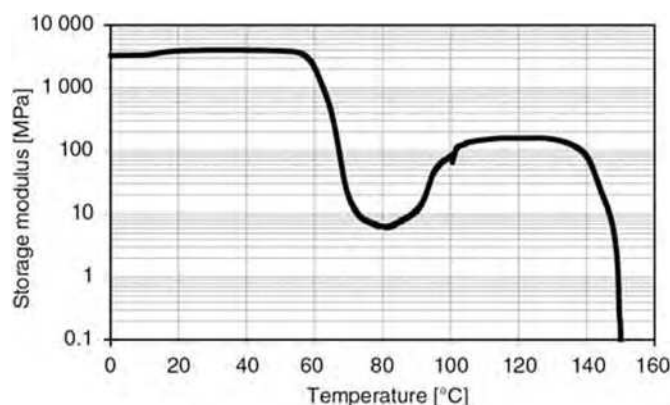
Fig. 7. The storage modulus of injection-molded PLA specimen (reprinted from “T. Tábi, I.E. Sajó, F. Szabó, A.S. Luyt, J.G. Kovács, Crystalline structure of annealed polylactic acid and its relation to processing, Express Polym. Lett. , 4 (2010), 659–668”, Copyright (2010), with the permission from Express Polymer Letters).
