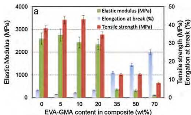
Fig. 22. Mechanical properties of PLA/Elvaloy (EVA-GMA) blends (reprinted from “M. Pracella, M.M.-U. Haque, M. Paci, V. Alvarez, Property tuning of poly (lactic acid)/cellulose bio-composites through blending with modified ethylene-vinyl acetate copolymer, Carbohydr. Polym., 137 (2016), 515–524”, Copyright (2016), with the permission from Elsevier).
