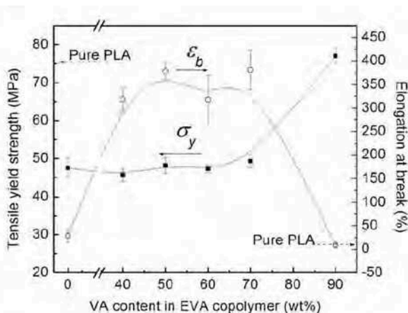
Fig. 18. Mechanical properties of PLA/EVA (80/20 wt%) blends in a function of VA content (reprinted from “P. Ma, D.G. Hristova-Bogaerds, J.G.P. Goossens, A.B. Spoelstra, Y. Zhang, P.J. Lemstra, Toughening of poly(lactic acid) by ethylene-co-vinyl acetate copolymer with different vinyl acetate contents, Eur. Polym. J., 48 (2012), 146–154”, Copyright (2012), with the permission from Elsevier).
