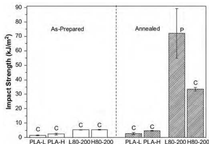
Fig. 23. Impact strength of not crystallized and crystallized PLA with 20 wt% of EGMA content. PLA-L and PLA-H refers to low and high M_w PLA grades (reprinted from “H.T. Oyama, Super-tough poly(lactic acid) materials: Reactive blending with ethylene copolymer, Polym., 50 (2009), 747–751”, Copyright (2009), with the permission from Elsevier).
