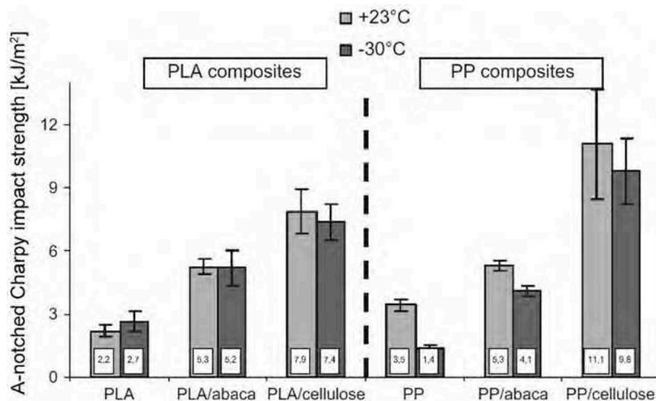
Fig. 37. Charpy impact strength of natural fiber reinforced, injection-molded PLA biocomposites (reprinted from “A.K. Bledzki, A. Jaszkievicz, D. Scherzer, Mechanical properties of PLA composites with man-made cellulose and abaca fibres, Compos. Part A Appl. Sci. Manuf. , 40 (2009), 404–412”, Copyright (2009), with the permission from Elsevier).
