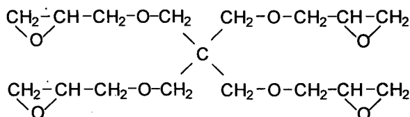
Eporezit AH-16
