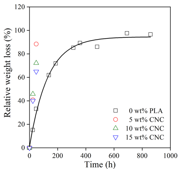
Fig. 8. Relative weight loss of PLA samples measured during their enzymatic degradation in the presence of proteinase K. Symbols: (□) neat PLA, (○) 5, (△) 10, (▼) 15 wt% crystalline nanocellulose (pH = 8.6, I = 25 mM).
