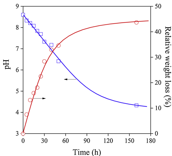
Fig. 3. Effect of pH on the degradation (weight loss) of neat PLA. Decreasing rate below pH = 6.5. Symbols: (○) weight loss, (□) pH. (initial pH = 8.6, I = 12 mM).
