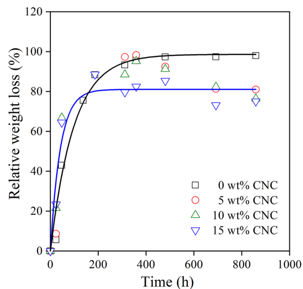
Fig. 9. Relative weight loss calculated from the results of UV-vis measurements plotted against the time of enzymatic degradation. Symbols are the same as in Fig. 8.
