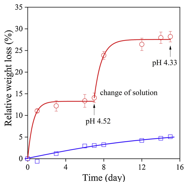
Fig. 2. Catalytic action of proteinase K in the degradation of neat PLA. Effect of pH and the changing of the degradation medium. Symbols: (○) with enzyme, (□) buffer (pH = 8.6, I = 12 mM).
