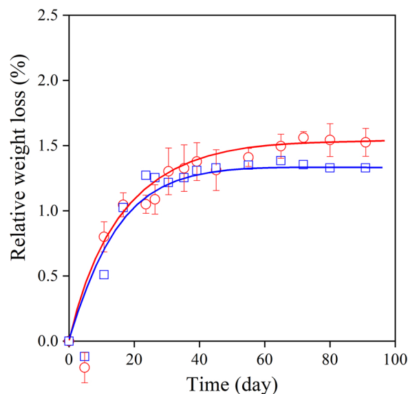
Fig. 1. Weight loss of neat PLA in the presence of CRL. Symbols: (○) with enzyme, (□) buffer (pH = 7.2).
