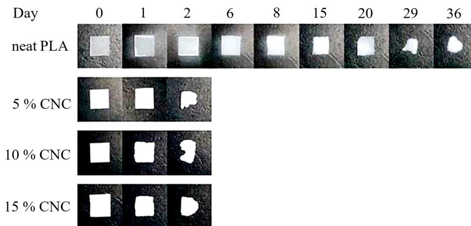
Fig. 5. Changes in the appearance of neat PLA and disintegration of the PLA/CNC composites during their enzymatic degradation ( \text{pH} = 8.6 , I = 25 \text{ mM} ).
