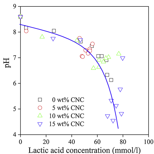
Fig. 10. pH of the degradation solution plotted against its lactic acid concentration. Non-linear correlation due to changing buffer capacity. Symbols are the same as in Fig. 8.
