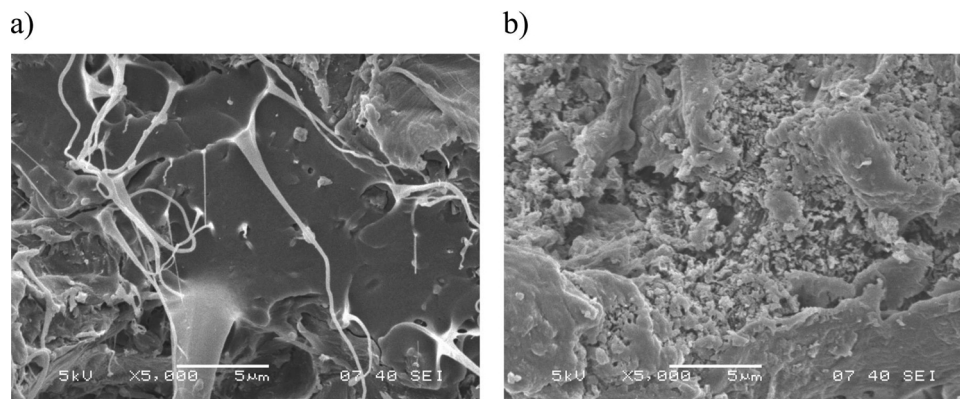
Fig. 6. SEM micrographs recorded on the fracture surface of the PLA/CNC nanocomposite containing 15 wt% CNC a) before degradation and b) after 48 h of enzymatic degradation ( \text{pH} = 8.6 , I = 25 \text{ mM} ).
