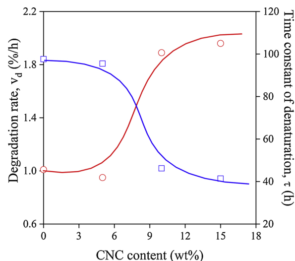
Fig. 11. Effect of CNC content on the rate of degradation and the time constant of denaturation during the enzymatic degradation of PLA/CNC nanocomposites. Symbols: (○) rate of degradation, v_d ; (□) time constant of denaturation, \tau (see Eq. 1).
