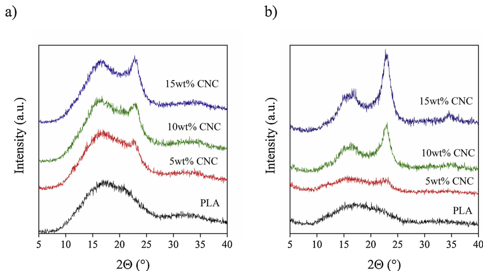
Fig. 7. XRD traces of neat PLA and that of the CNC nanocomposites a) before the start of the degradation experiments and b) after 48 h degradation (pH = 8.6, I = 25 mM).
