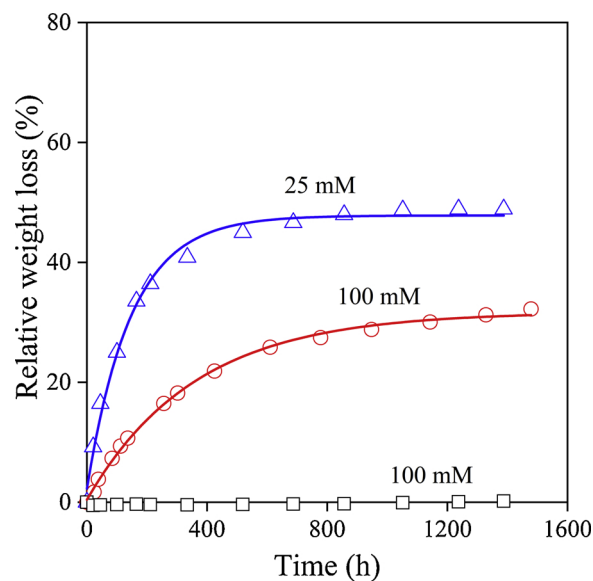
Fig. 4. Influence of the ionic strength of the buffer solution on the enzymatic activity of proteinase K. Symbols: (△) enzyme, I = 25 mM, (○) enzyme, I = 100 mM, (□) buffer, I = 100 mM (pH = 8.6).
